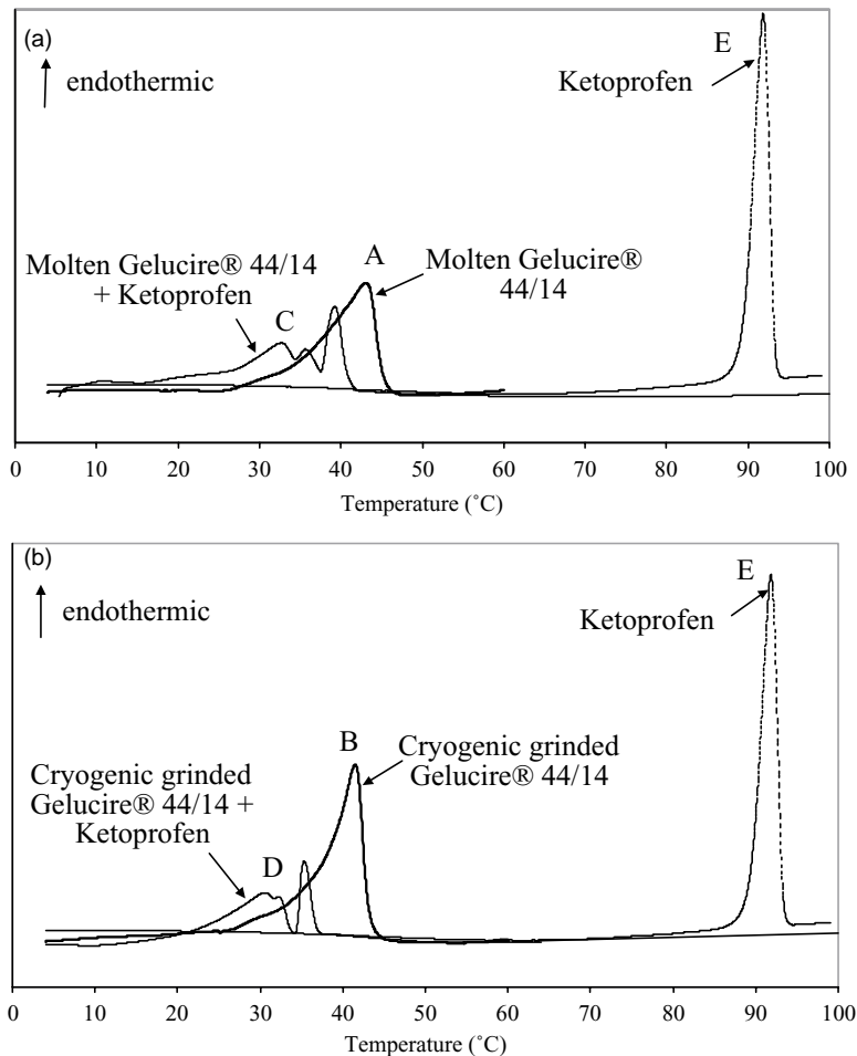
Fig. 2. Thermograms of molten Gelucire ® 44/14 (a) and cryogenic grinded Gelucire ® 44/14 (b).
