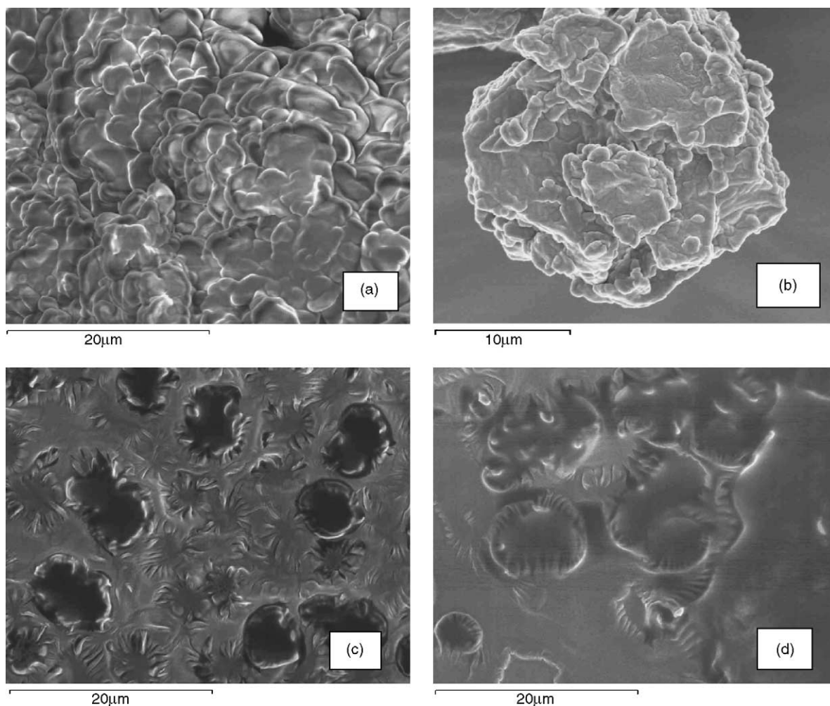
Fig. 1. Scanning electron micrographs (3000 \times ) of molten Gelucire ® 44/14 (a), cryogenic grinded Gelucire ® 44/14 (b), molten Gelucire ® 44/14/ketoprofen mixture (c) and cryogenic grinded Gelucire ® 44/14/ketoprofen mixture (d).
