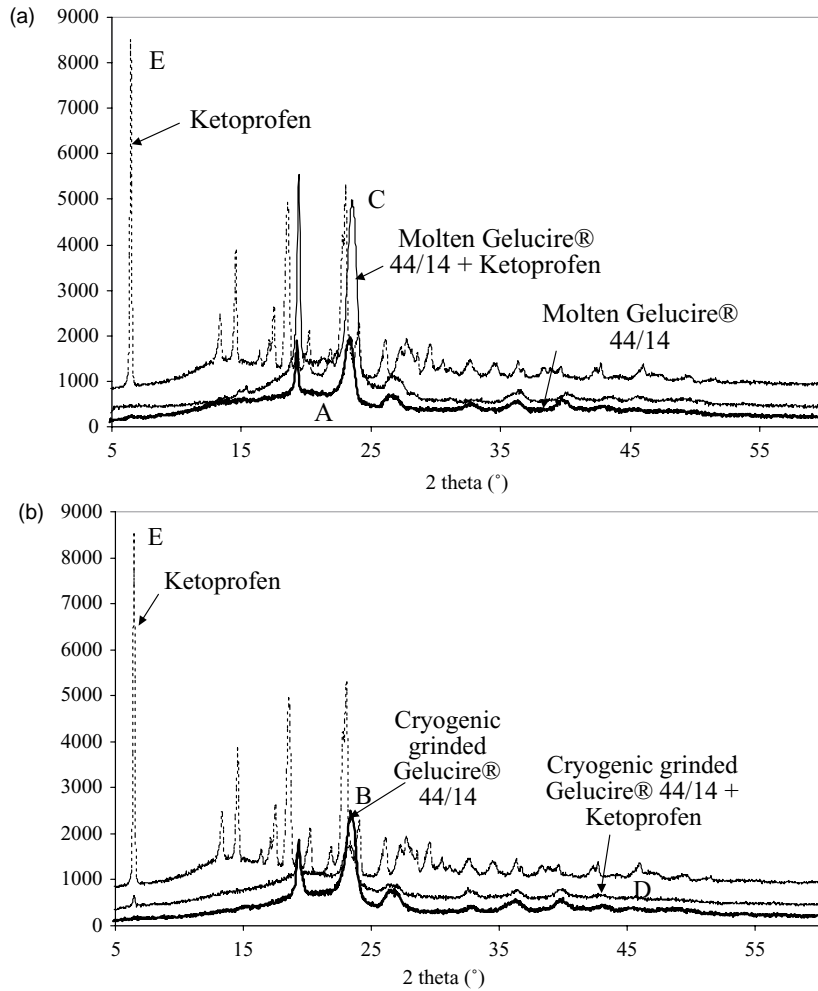
Fig. 3. X-ray patterns of molten Gelucire® 44/14 (a) and cryogenic grinded Gelucire® 44/14 (b).
