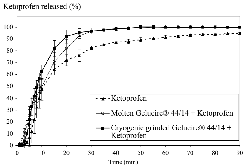
Fig. 6. Dissolution profiles obtained with ketoprofen (Topfena ® capsules), molten Gelucire ® 44/14/ketoprofen mixture and cryogenic grinded Gelucire ® 44/14/ketoprofen mixture.
